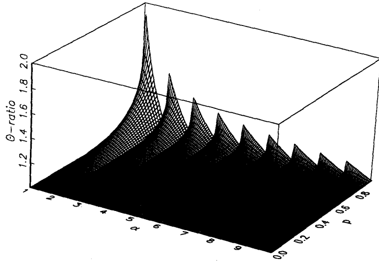
Fig. 1. The effect of \Theta^{n-1}(\alpha - \bar{n}, p) / \Theta^n(\alpha - \bar{n}, p) for 1 \leq \alpha \leq 10 and 0 \leq p \leq 1 . The effect of \Theta^{n-1}(\alpha - \bar{n}, p) / \Theta^n(\alpha - \bar{n}, p) on \alpha p decreases exponentially as p decreases, decreases in each interval \bar{n} - 1 < \alpha \leq \bar{n} as \alpha \rightarrow \bar{n} , and decreases exponentially overall as \alpha \rightarrow \infty .
