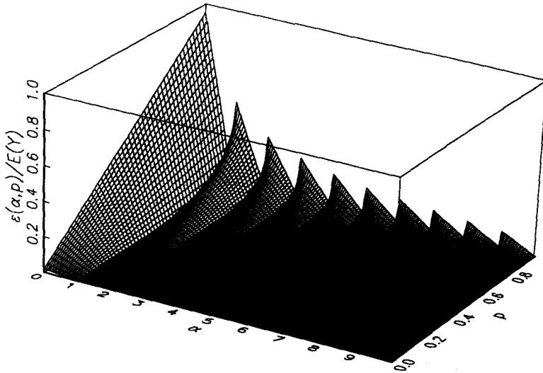
Fig. 3. Ratio of the error \epsilon(\alpha,p) to the expected value E(Y|\alpha,p) for 0 \leq \alpha \leq 10 and 0 \leq p \leq 1 . The ratio of the error \epsilon(\alpha,p) to the expected value E(Y|\alpha,p) is greatest for 0 < \alpha < 1 . Therefore, it (1) decreases exponentially as p decreases, (2) decreases in each interval \bar{n} - 1 < \alpha \leq \bar{n} as \alpha \rightarrow \bar{n} , and (3) decreases exponentially overall as \alpha \rightarrow \infty .
