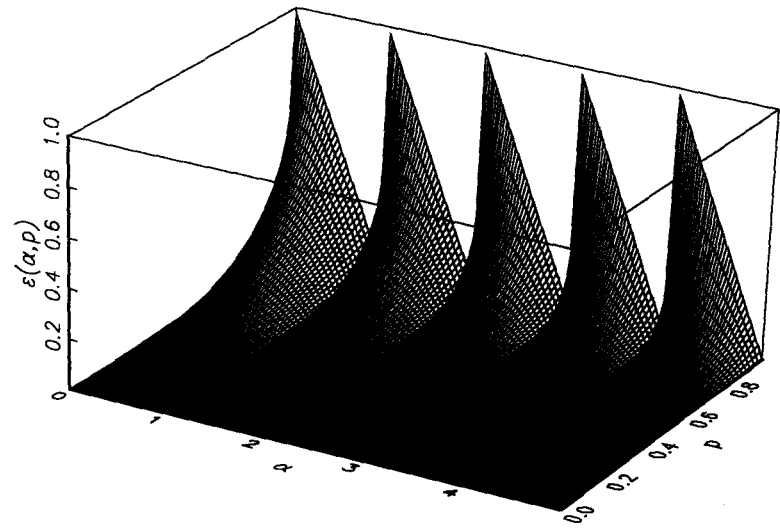
Fig. 2. Plot of the error \epsilon(\alpha, p) = E(Y|\alpha, p) - \alpha p for 0 \leq \alpha \leq 5 and 0 \leq p \leq 1 . The error decreases exponentially as p decreases, decreases in each interval \bar{n} - 1 < \alpha \leq \bar{n} as \alpha \rightarrow \bar{n} , and decreases overall as \alpha \rightarrow \infty .
