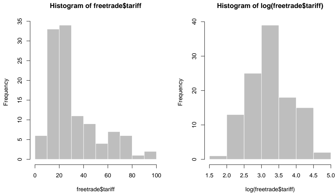
Figure 3: Histogram of tariff and log(tariff) .
