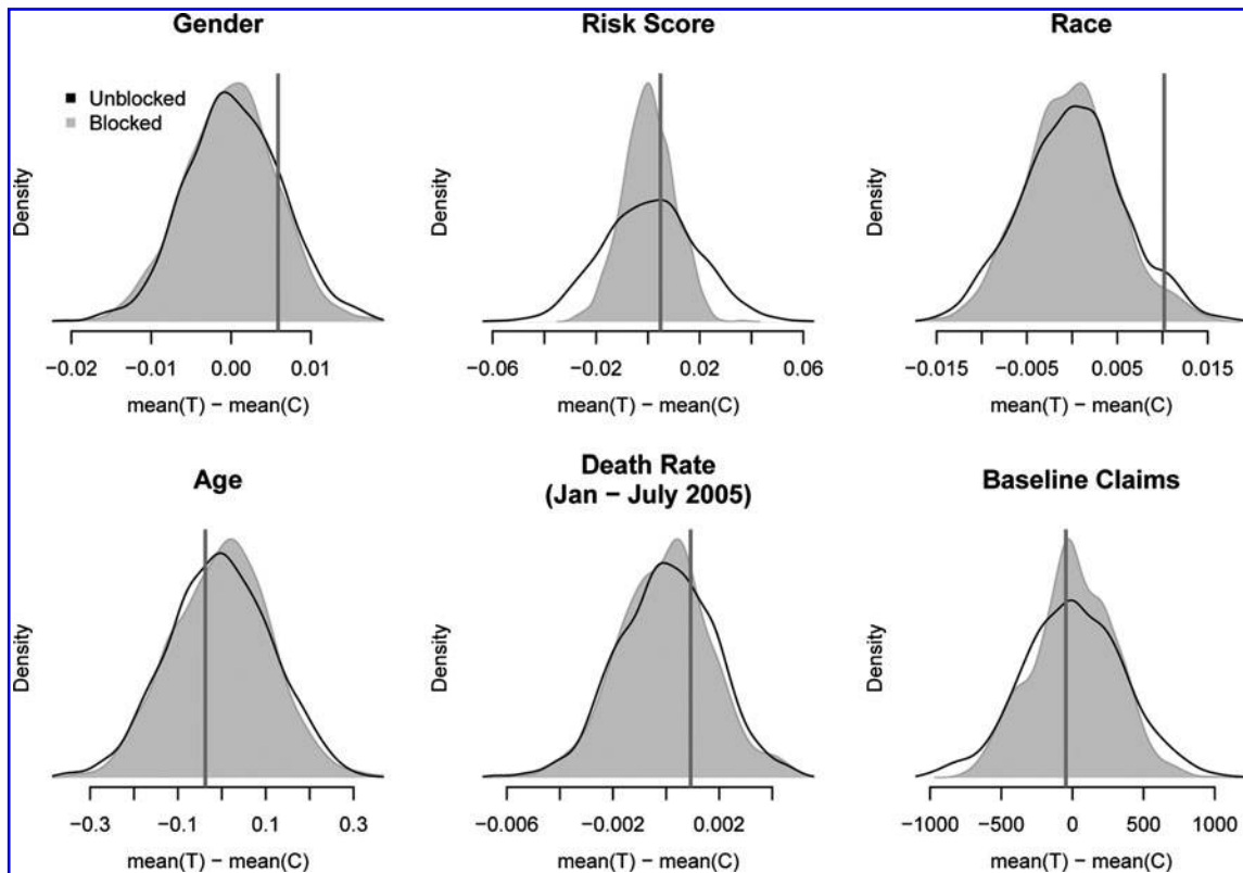
FIG. 2. Randomization distributions, for the actual blocked experiment ( gray ) and under complete randomization ( black ), with a vertical line representing the one actual randomization assignment. Note that the horizontal range, and thus the meaning of the distance from the vertical line from the zero point, of each variable differs.
