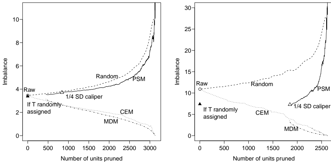
Figure 3: Imbalance-Matched Sample Size Graph, with data from Finkel, Horowitz, and Rojo-Mendoza (2012) for the left panel and Nielsen, Findley, et al. (2011) for the right.
